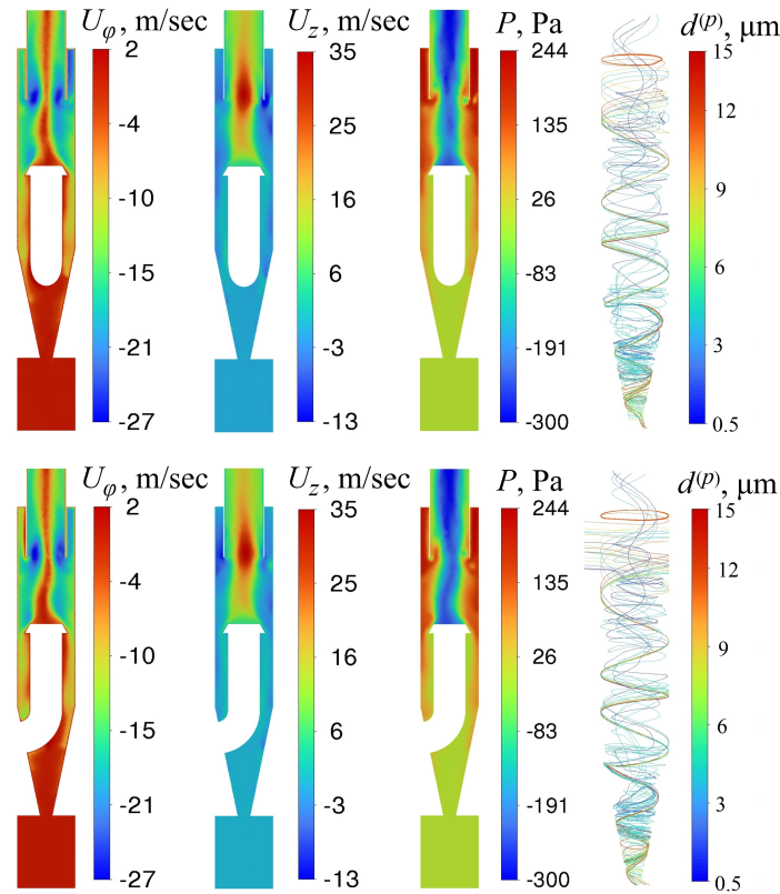
Fig. 6. Distribution of physical characteristics in the CCSS where the upper row shows the pressure, azimuthal velocity, vertical velocity, and solid particle trajectories in the xz plane, and the lower row relates to the yz plane
