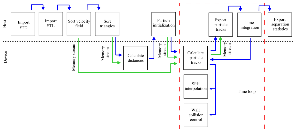
Fig. 2. Interaction scheme between the central processing unit and the graphics accelerator
