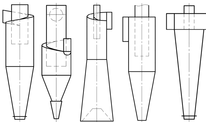
Fig. 4. Examples of different designs of classic cyclones [6]
