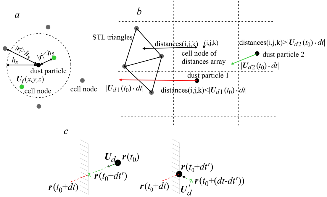
Fig. 3. Interaction scheme of a particle with irregular meshes: a – interpolation of the gas velocity field at the particle position using an SPH filter, b – criteria for initiating the collision check between a particle and a solid wall, c – processing of a triangle intersection by a particle displacement vector using local time-step truncation
