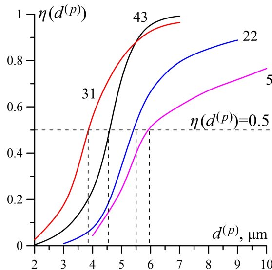
Fig. 7. Examples of fractional efficiencies for some points of the hypercube
