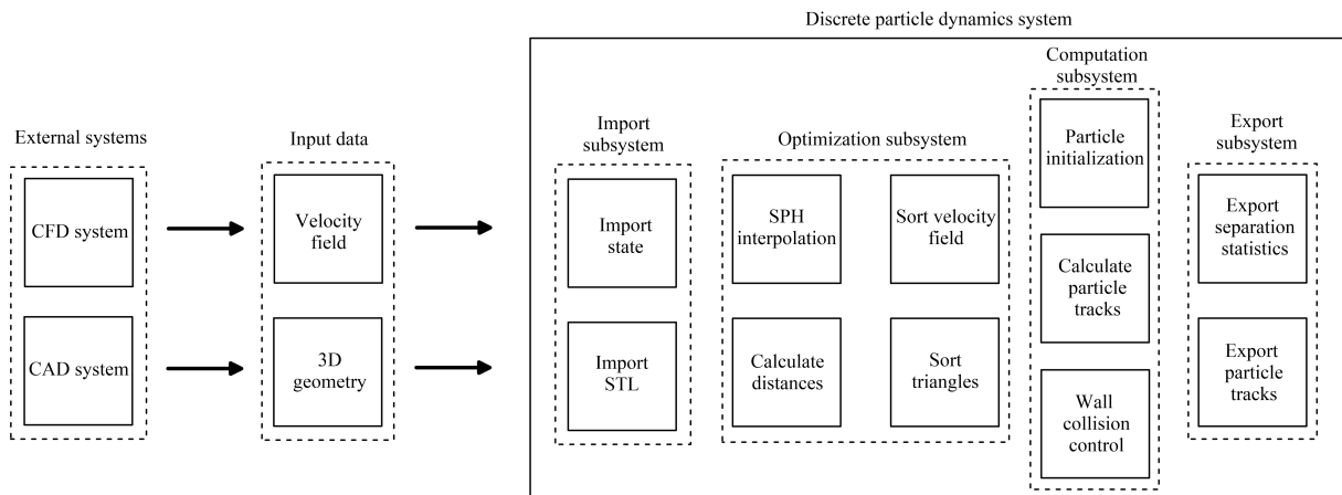
Fig. 1. Software architecture for discrete particle dynamics modeling within a gas velocity field trajectory calculations, the final stage performs the export of separation statistics.
