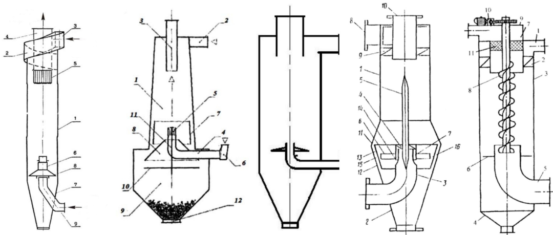
Fig. 5. Examples of different CCSS constructs [1]
